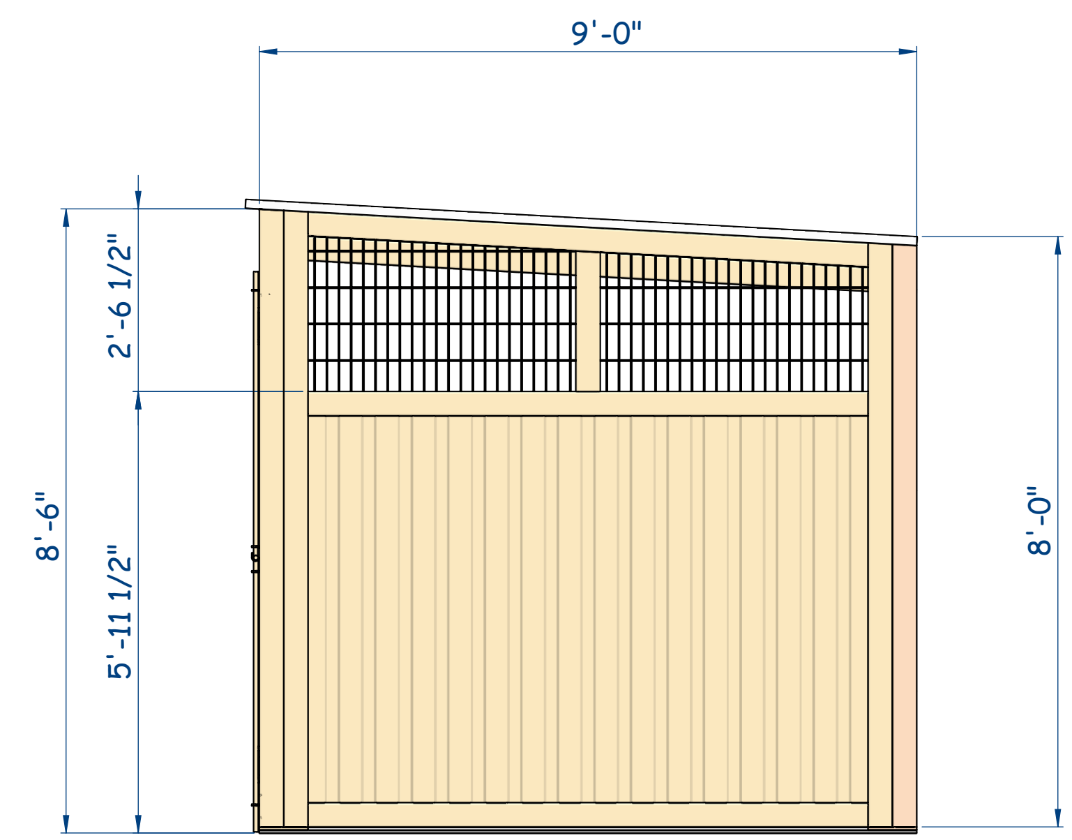
SIDE ELEVATION
