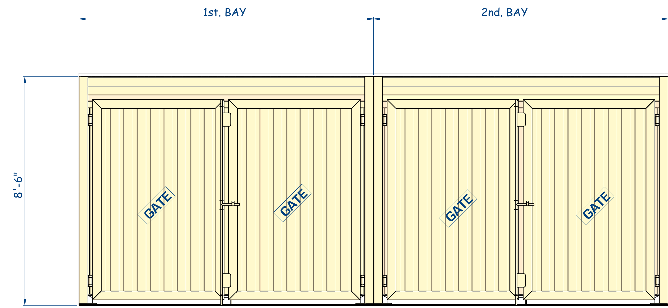
FRONT ELEVATION
