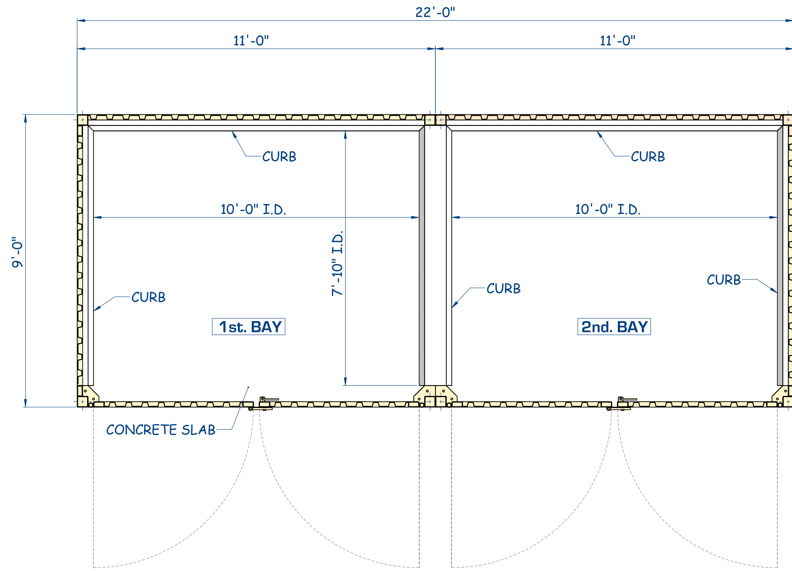
FLOOR PLAN
